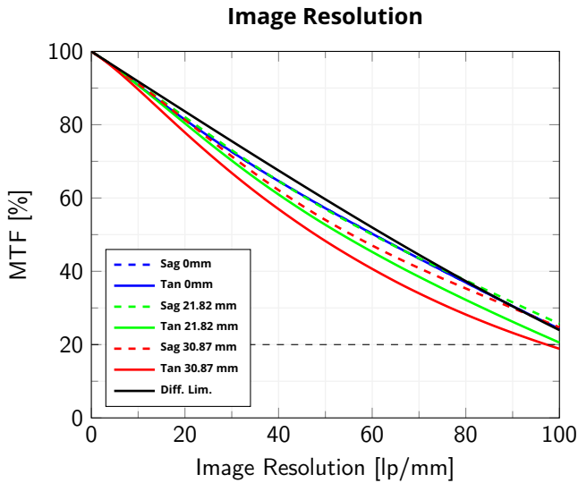
Modulation Transfer Function (MTF) vs. Image Resolution, wavelength range 460-630 nm, wf/N = 11
