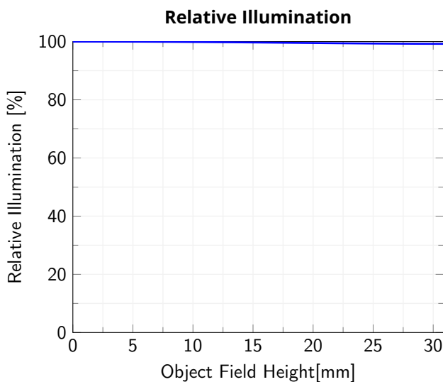
Relative illumination vs. Object Field Height, from the optical axis to the corner of the field of view, wf/N = 11
