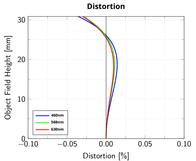
Object Field Height vs. Distortion, from the optical axis to the corner of the field of view, wf/N = 11
