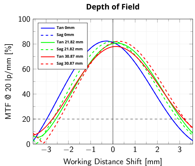
Modulation Transfer Function (MTF) @ 20 lp/mm vs. Working Distance Shift from the best focus Working Distance, wavelength range 460-630 nm, wf/N = 11
